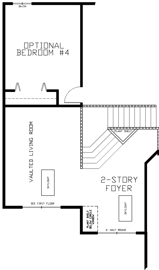
OPTIONAL STAIRS/BEDROOM #4
